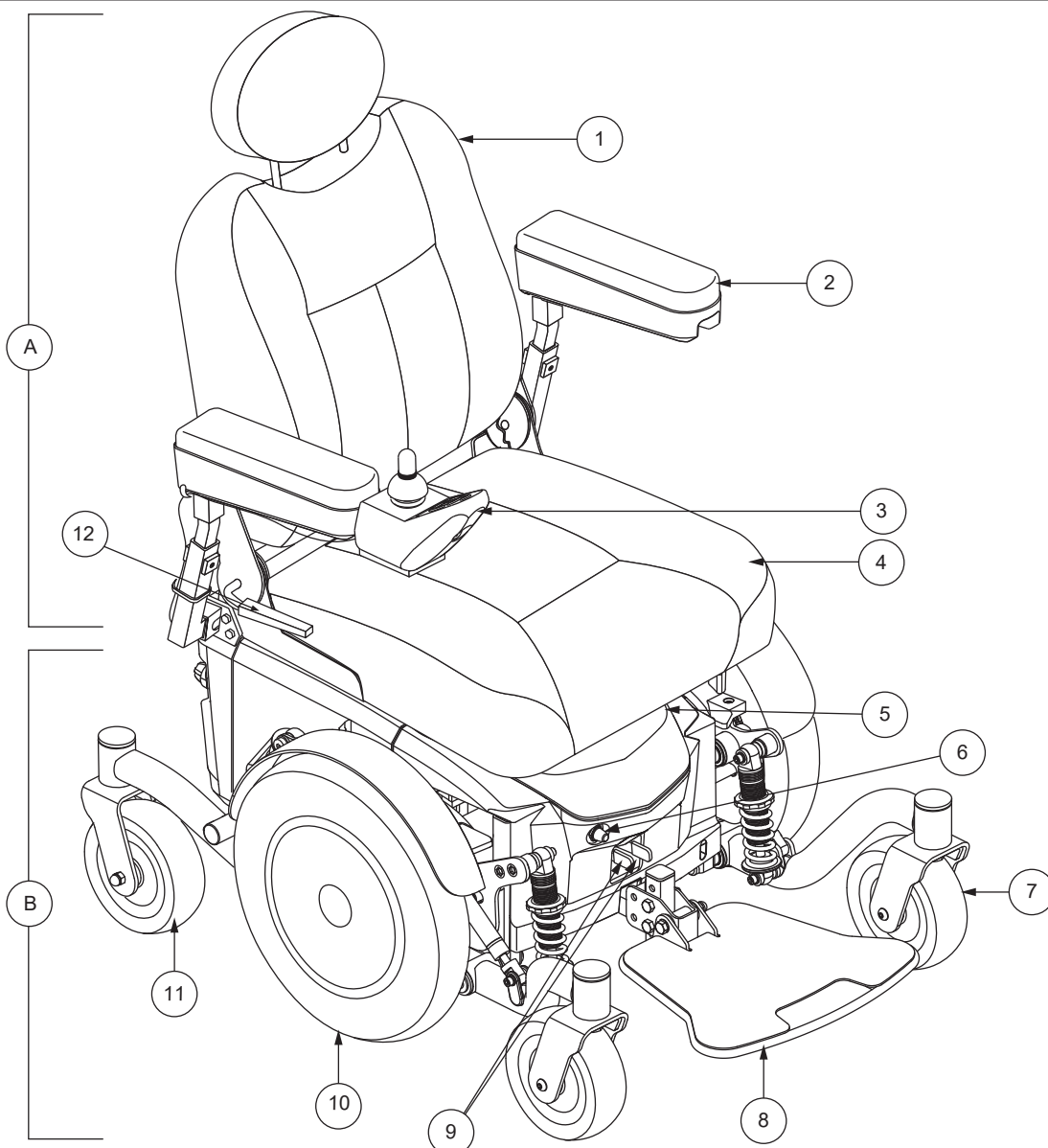
Figure 1. The Jazzy EVO 614 Series Power Chair
