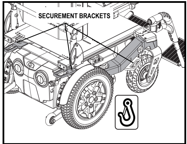
Figure 7. Transit System Securement Brackets
