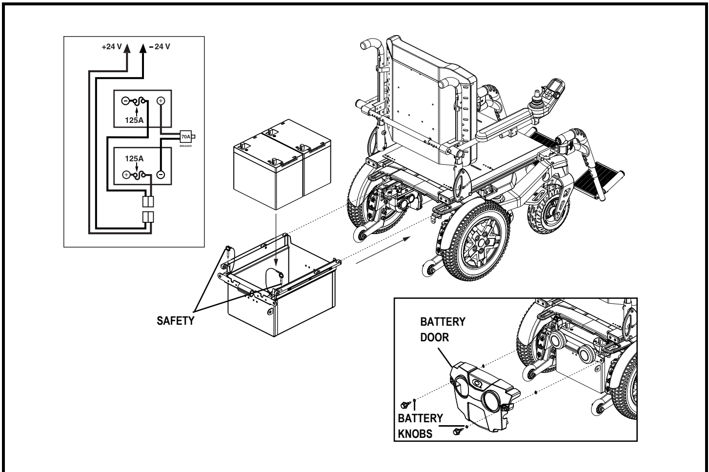
Figure 20. Battery Replacement
