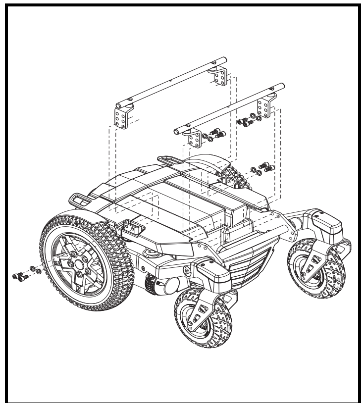
Figure 11. Seat Height/Angle Adjustment
