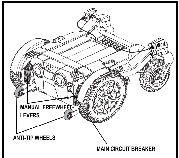
Figure 6. The Rival Power Base
